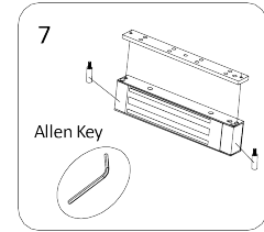
Use Allen key to remove the mounting plate from lock body.
