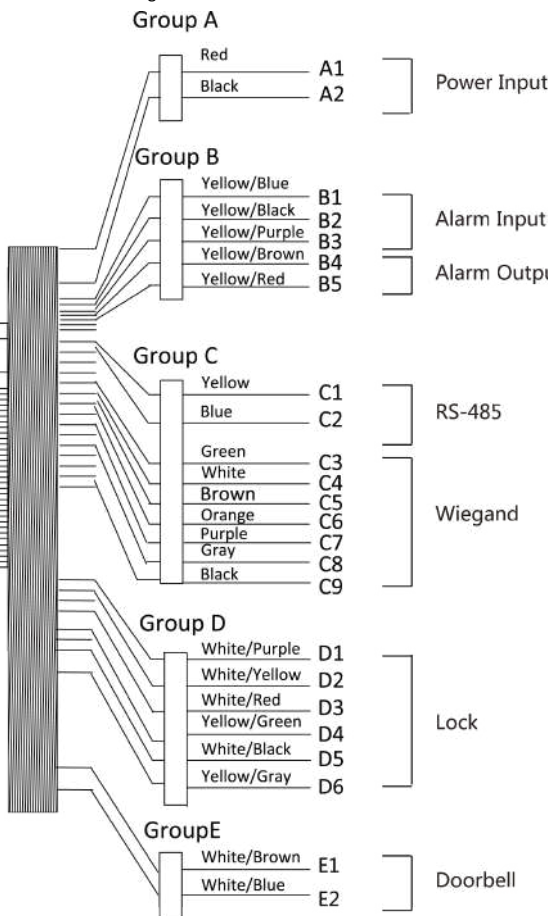
Figure 4-1 Terminal Diagram
